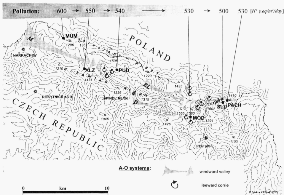
Fig. 1. – Location of the examined six plots in the Giant Mts., the Sudetes with regard to the A-O systems of Mumlava M, Bílé Labe BL and Dlouhý Důl D (Jeník 1961). Decreasing gradient of acidifying deposition ( H^+ in throughfall between June 2 and November 4, 1994) is given according to Hošek & Kaufman (1995). Plots: MUM – Mumlavská Mt, ALZ – Alžbětinka, PUD – Pudlava, MOD – Modrý důl valley, SLU – Slunečné údolí valley, PACH – Pašerácký chodník.
