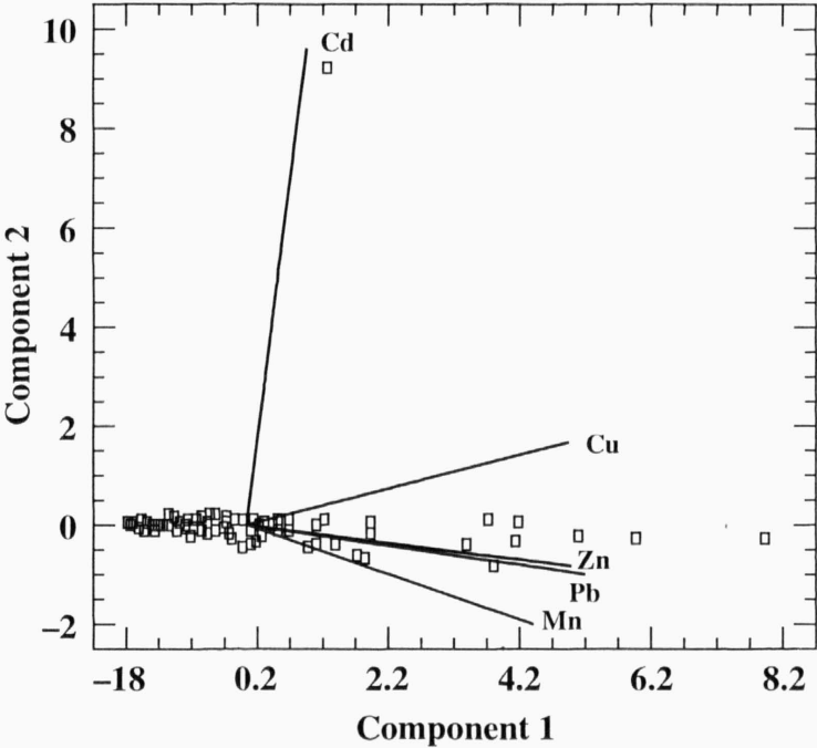
Fig. 2. – PCA ordination of the complete analytical data set along the two first variability componnets.
