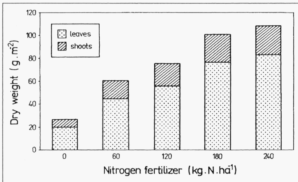
Fig. 3. – Leaf and shoot yield ( \text{g.m}^{-2} ; mean value of both days of harvest) of Urtica dioica in dependence on addition of nitrogen-fertilizer (in kg of N per hectare) (from Weiss 1993, adapted).
