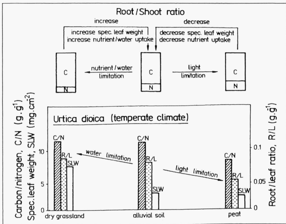
Fig. 4. – Scheme of regulatory responses to light, water and nutrient limitations leading to a balanced resource supply (top part). Change of the carbon/nitrogen ratio (C/N), root weight/leaf weight ratio (R/L), and specific leaf weight (SLW) in Urtica dioica in Bayreuth, Germany (from Schulze & Chapin III 1987, adapted).
