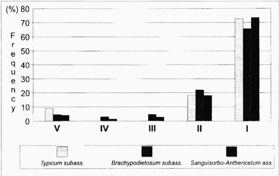
Fig. 2. – Presence histogram of the Sanguisorbo-Anthericetum species.
