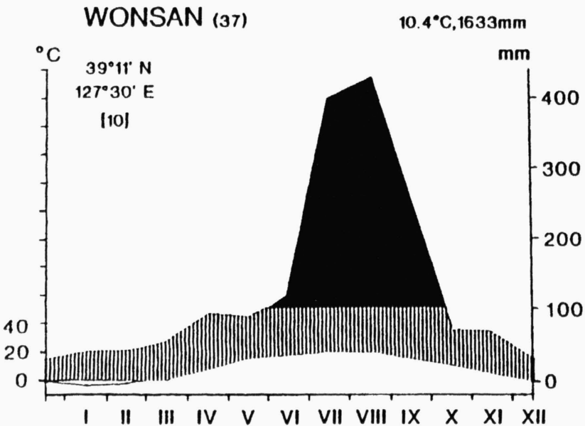
Fig. 1. – Climatic characteristics of Wonsan situated ca. 80 km NW from Kumgangsan Mts. (according to Krebs et al. 1984, modified).
