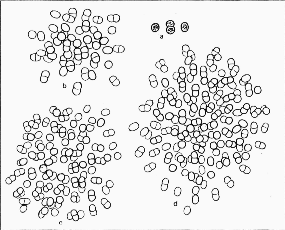
Fig. 1. - Radiocystis fernandoi , spec. nova (iconotype).
