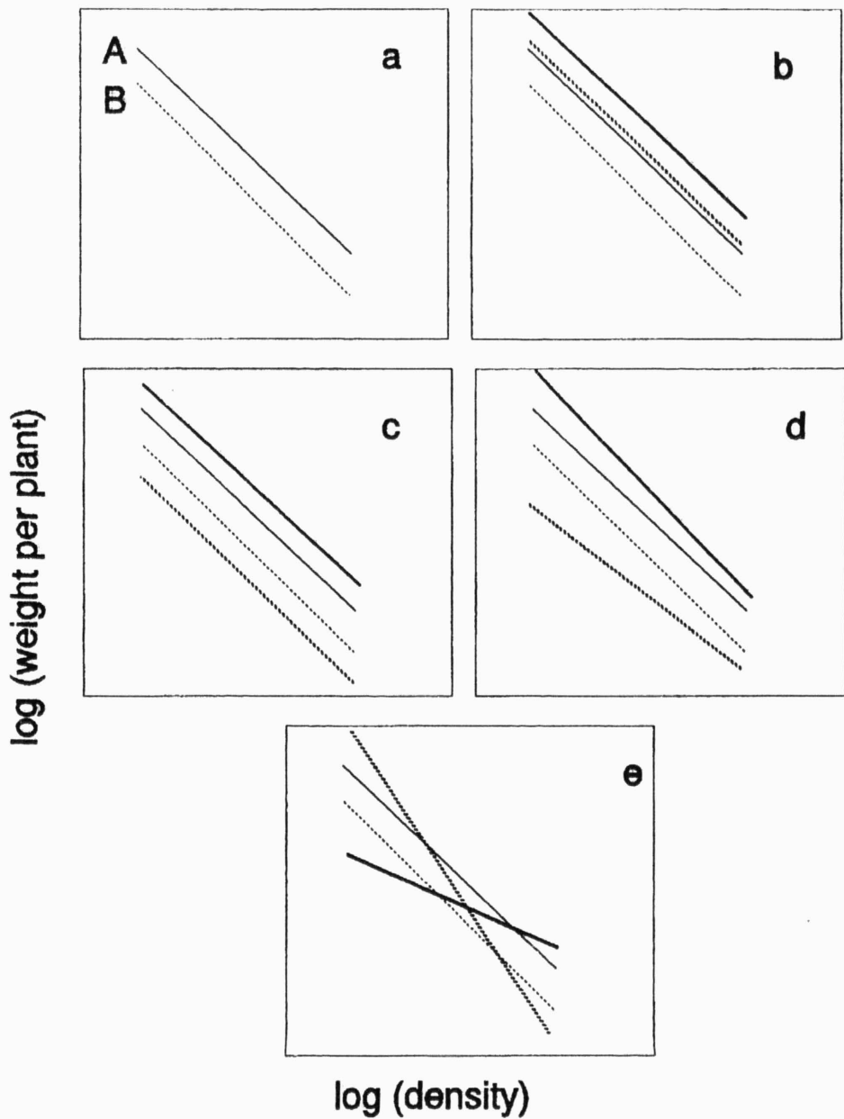
Fig. 4. - Thinning of species A (solid line) and B (dashed line) in monoculture (graphic a and thin lines of graphs b-e) and in mixtures (thick lines of graphs b-e) assuming different levels of resource-use overlap and competitive ability (see text for description).
