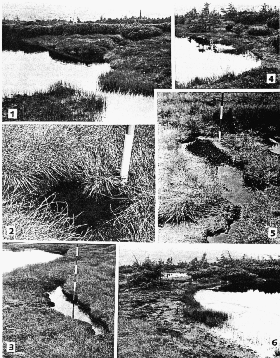
Fig. 4. Elements of microtopography and vegetation on Pančava Mire; 1 - bog pool No. 3 surrounded by the Chamaemoro-Pinetum mughii , 2 - embryonic pool between the tussocks of Eriophorum vaginatum , occupied by Gymnocolea inflata , 3 - pool elongated along the contour line, 4 - bog pool No. 2 fringed by a sunken bank, 5 - desiccating pool whose floor is partly disintegrated by larvae of Chironomidae , 6 - bog pool No. 1 fringed by a belt of Carex limosa (lake No. 2 in background); for situation and general characteristics of bog pools see Fig. 2 and Table 1.
