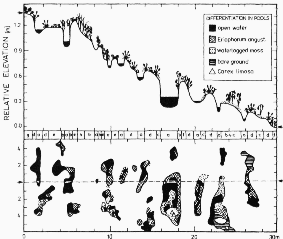
Fig. 7. - Ground plan (bottom) and cross-section (top) of a string-and-flark mire in the SW part of Pančava Mire; its situation see in Fig. 2. Phytosociological composition along the transect is indicated as follows - a: microalgal communities, b: Calliergo sarmentosi-Eriophoretum vaginati , c: Sphagno dusenii-Caricetum limosae , d: Eriophoro vaginati-Polytrichetum stricti , e: Chamaemoro-Empetretum hermaphroditii , f: Sphagno robusti-Empetretum hermaphroditii , g: Chamaemoro-Pinetum mughi , h: Polytricho communis-Molinietum caeruleae .
