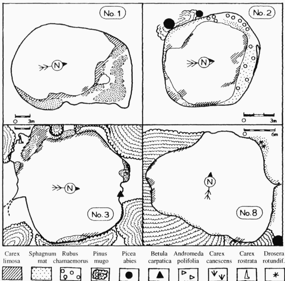
Fig. 6. - Ground plan and vegetation of four mire pools on Pančava Mire; for numbers and situation of the pools see Fig. 2. and Table 1. Vegetation pattern indicates main stands with respective dominants. Recorded on July 3, 1992.
