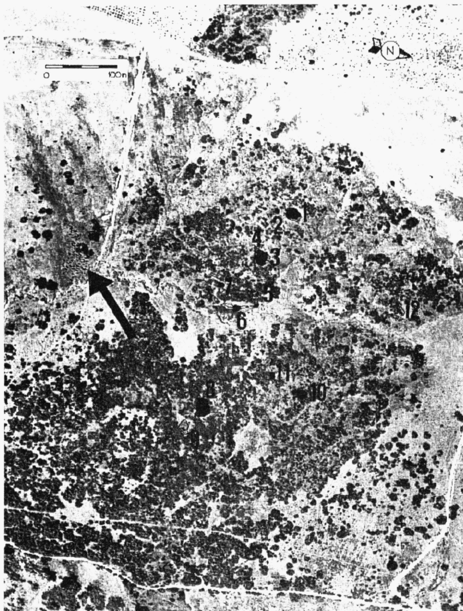
Fig. 2. Aerial photograph of Pančava Mire taken on July 30, 1958; the numbers refer to the bog pools (black spots) listed in Table 1; large arrow points out the string-and-flark system analyzed in Fig. 7.
