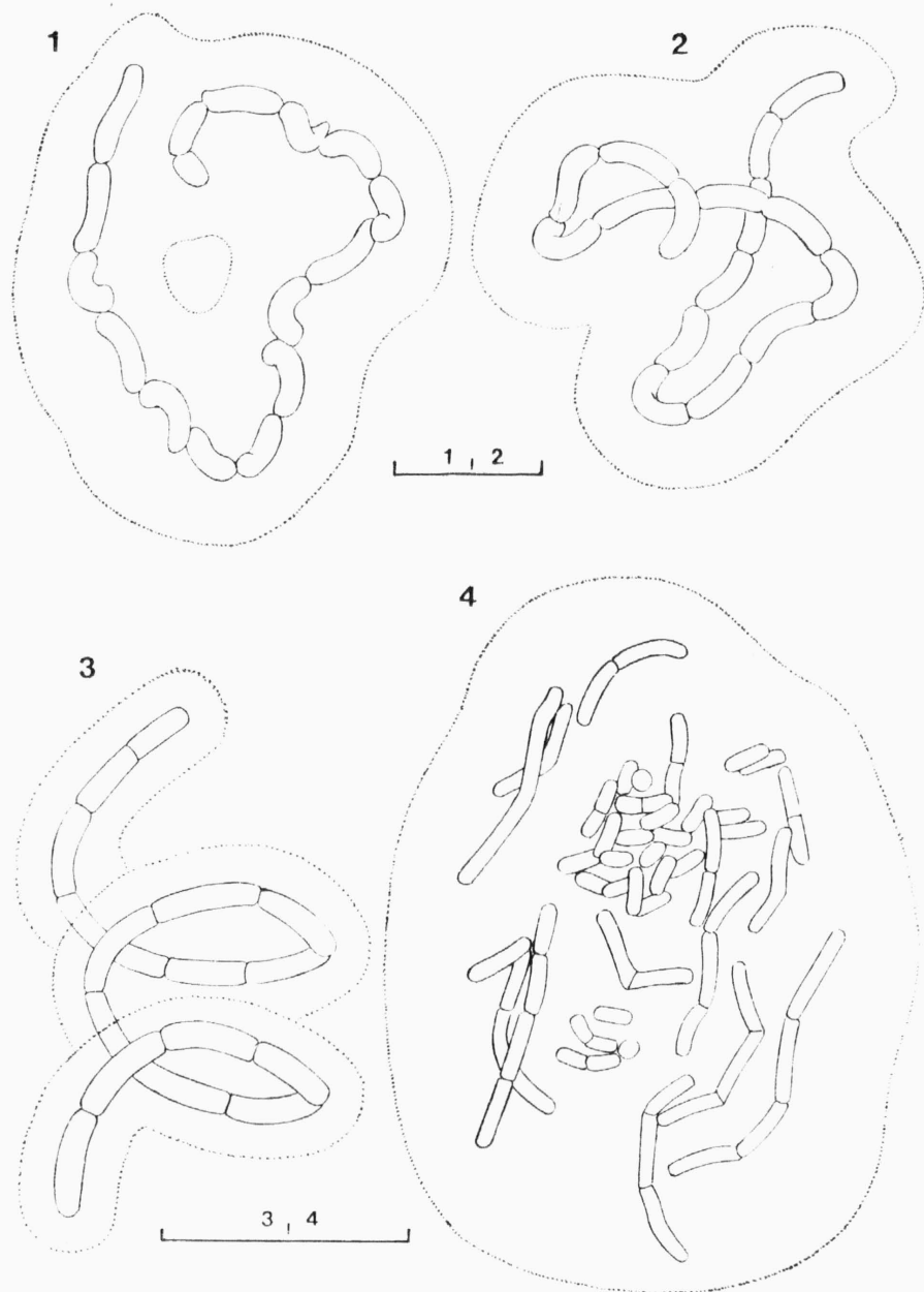
Fig. 4. — 1, 2, Romeria simplex (HIND.) HIND., specimens from a gravel pit lake at Medvedov, 3, R. okensis (MAYER) HIND., a pseudofilament from the River Danube in Bratislava, 4, Rhabdoderma linearis SCHMIDLE et LAUTERB., a colony from a water reservoir at Boleráz near Trnava. Scale: 10 \mu m.
