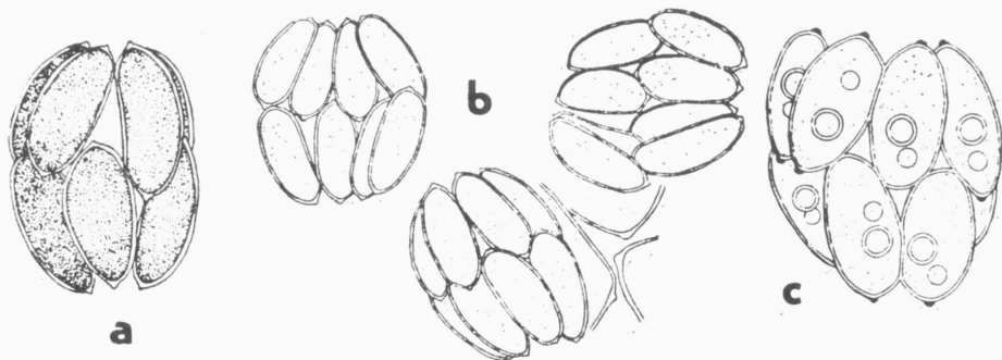
Fig. 9. — Steinedesmus capitatus (G. M. SMITH) comb. nova: a iconotype of Sc. arcuatus var. capitatus G. M. SMITH 1918 from USA, b after G. M. SMITH 1920, c after HORTOBÁGYI 1969 from India.
