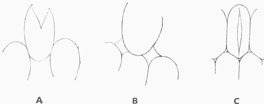
Fig. 2. — Disintegration patterns of the mother cell walls in Steinedesmus — A, Rayssiella — B, and Scenedesmus (subg. Scenedesmus ) — C. (Orig.)
