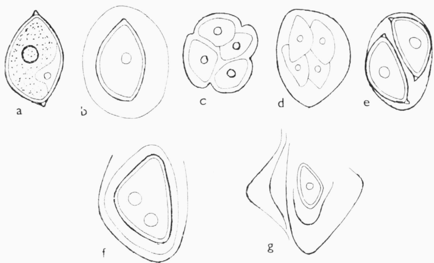
Fig. 11. — Ecdysichlamys obliqua G. S. WEST; a = cell, b = daughter cell in the mother cell wall, c — e = autospore formation, f — g = liberation of daughter cells from the lamellated mother cell wall (according to G. S. WEST 1912).
