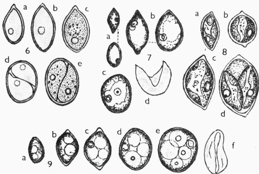
Fig. 6. — Ecdysichlamys alpina (REISIGL) comb. nova; a–c = solitary cells, d–e = autospore formation (according to REISIGL 1964).
