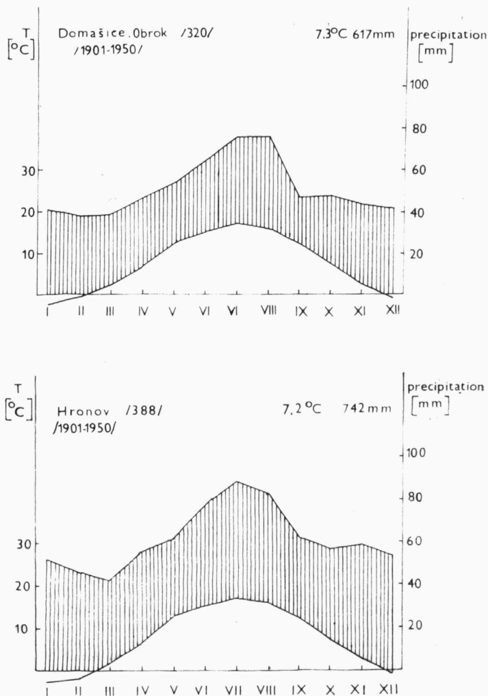
Fig. 3. Climatic diagrams representing two climatic regimes of sandstone areas (based on data in Vesecký et al. 1958).
