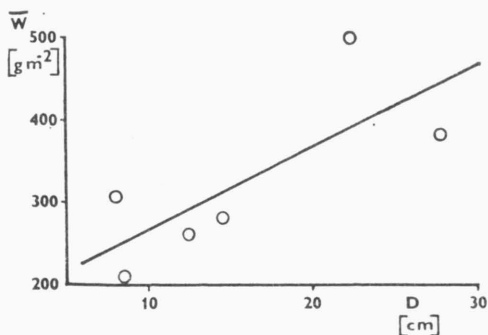
Fig. 4. — Regression curve of the dependence of aboveground living maximum biomass ( \bar{W} mean dry mass of three seasons) /\text{g m}^{-2}/ on the depth of A soil horizon ( D ) /\text{cm}/ .
