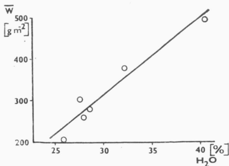
Fig. 3. — Regression curve of the dependence of aboveground living maximum biomass ( \bar{W} mean dry mass of three seasons) /\text{g m}^{-2}/ on mean year soil moisture ( \text{H}_2\text{O} ) /\% dry mass/.
