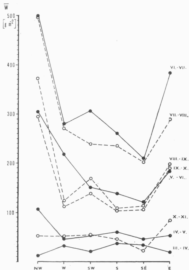
Fig. 5. — Changes in aboveground living biomass (W mean dry mass of three seasons) \text{g m}^{-2} on the isohypse transect with NW., W., SW., S, SE., E. orientation in month intervals. Fully line: month intervals from 15. 3. to 15. 6., dashed line: month intervals from 15. 7. to 15. 11.
