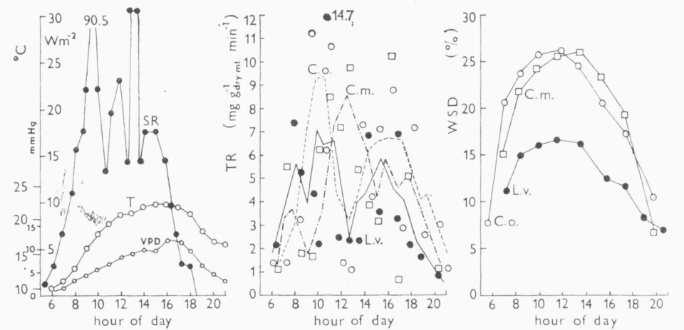
Fig. 2. — Daily courses of several microclimatic and shrub water-relation parameters in the oak-hornbeam forest at Báb (August 24). Left: Solar radiation (SR), air temperature (T) and vapour pressure deficit (VPD) at the height of 2 m within the forest canopy. Middle: Transpiration rate (TR, gliding averages and original data). Right: Water saturation deficit (WSD). Soil moisture content at the depth of 10 to 40 cm: 11.9 per cent. — C. o. = Crataegus oxyacantha (○, dotted line), C. m. = Cornus mas (□, - . - . -), L. v. = Ligustrum vulgare (●, full line)
