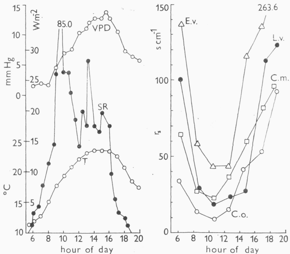
Fig. 4. — Daily courses of stomatal resistance for four species of shrubs growing in the oak-hornbeam forest at Báb (right), and of vapour pressure deficit (VPD), solar radiation (SR) and air temperature (T) at the height of 2 m within the forest canopy (left). (August 25). For legend see Fig. 1.
