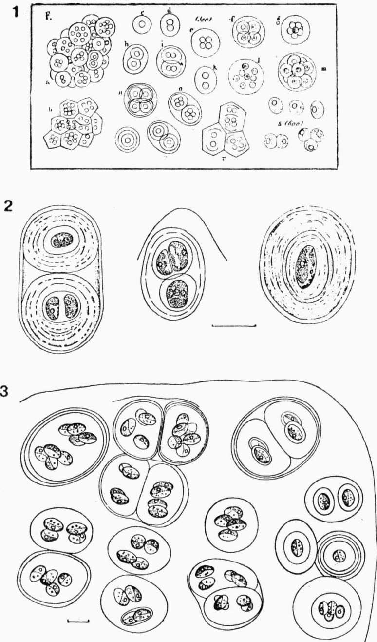
Fig. 2. — 1, Gloeocystis vesiculosa NÄG. (iconotype, from NÄGELI 1849). 2—3, G. polydermatica (KÜTZ.) HIND. [2, from VAN DEN HOEK 1963, as the type of Gloeocapsa polydermatica KÜTZ.; 3, from FOTT et NOVÁKOVÁ 1971, as Palmogloea protuberans (SMITH et SOW.) KÜTZ.; scale: 10 \mu m].
