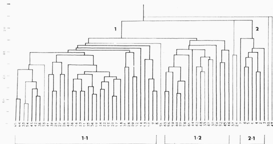
Fig. 12. Hierarchical dendrogram showing cluster relations among individual relevés of winter weed plant communities. (1 Meliloton indicis foed. nova; 1.1 Convolvulo (arvensis) - Rumicetum dentati ass. nova; 1.2 Astragalo (corrugati) - Plantaginetum lagopi ass. nova; 2 Achilleion santolinae ZOH. 1950; 2.1 Achilleetum santolinae mareoticum TADROS et ATTA 1958.)
