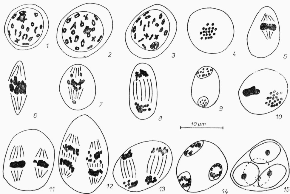
Abb. 3. — Anagallis foemina MILL., normaler Ablauf der Meiosis. — 1, 2, 3: Diakinese; 4, 5: Metaphase I; 6, 7, 8: Anaphase I; 9: Interkinese; 10, 11: Metaphase II; 12, 13: Anaphase II; 14: Tetradenkern; 15: Tetradenzellen.
