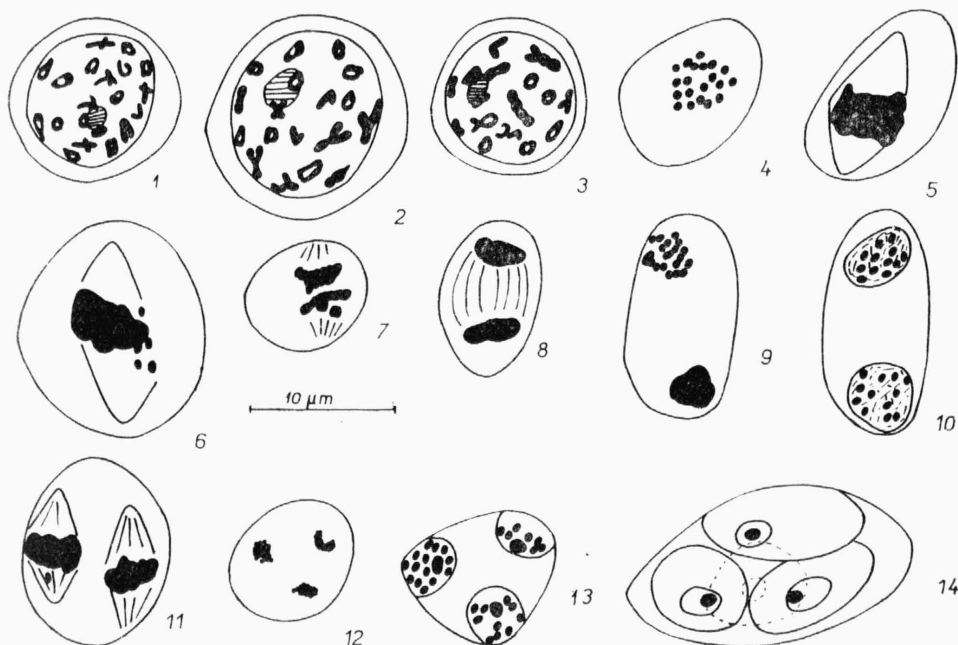
Abb. 2. — Anagallis arvensis L., normaler Ablauf der Meiosis. — 1, 2, 3: Diakinese; 4, 5, 6: Metaphase I; 7: Anaphase I; 8: Telophase I; 10: Interkinese; 9, 11: Metaphase II; 12: Anaphase II; 13: Tetradenkerne; 14: Tetradenzellen.
