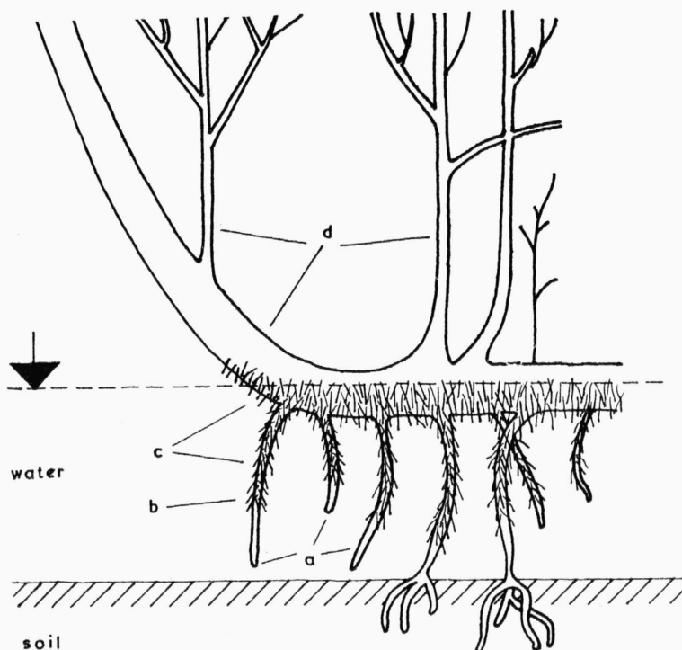
Fig. 1. Adventitious root system developed on the floating stems of Aeschynomene elaphroxylon ; a — macrorrhizae, b — skeleton roots developed from macrorrhizae, c — brachyrhizae, d — stems.
