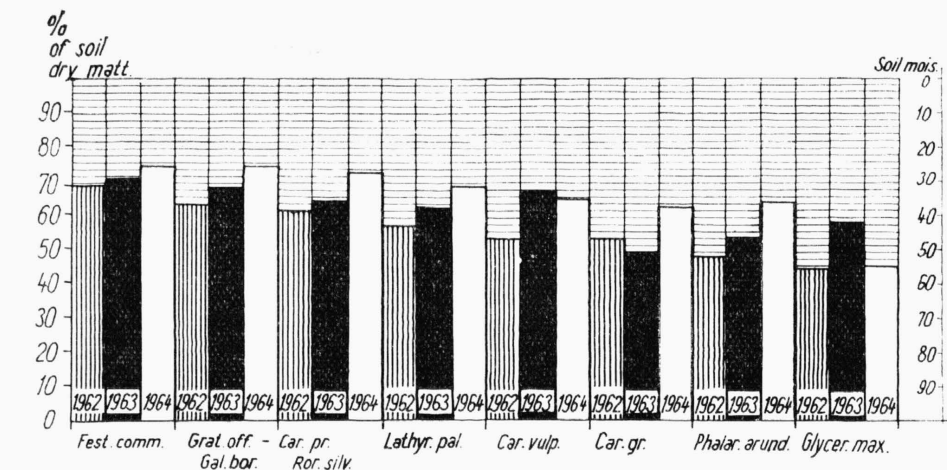
Fig. 2. — Averages of dry matter content of the soils in the eight plant communities studied for the years 1962 (hatched), 1963 (solid black) and 1964 (white). The numbering of plant communities as in Fig. 1. (horizontal line) soil moisture.
