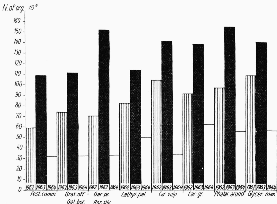
Fig. 3. — Averages of the numbers of all microorganisms in the soils under the plant communities studied in the years 1962 (hatched), 1963 (solid black) and 1964 (white). The numbering of the plant communities as in Fig. 1.
