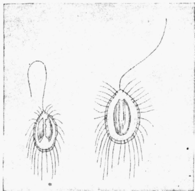
Fig. 2. — Iconotype of Mallomonas acaroides PERTY. — Reproduced from CONRAD 1927 after PERTY 1851.
