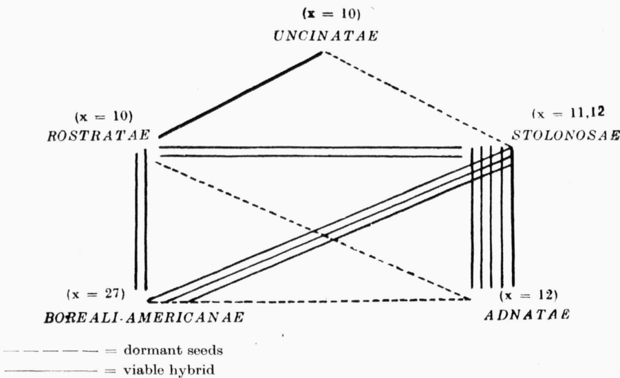
Figure 1 Artificial crosses and basic chromosome numbers in the section Nomimum (From GERSHOY, 1934, 1943)
